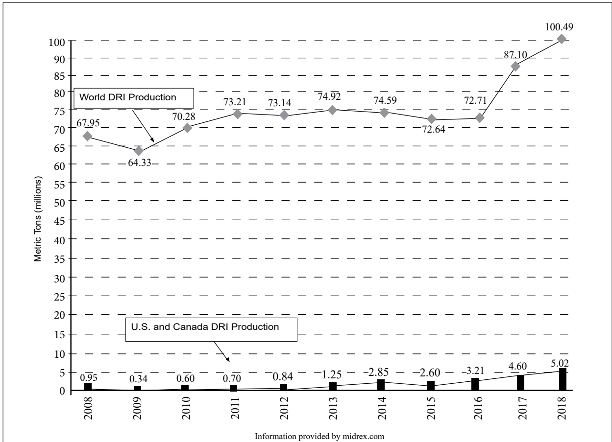
Figure 14 World Direct Reduced Iron Production
